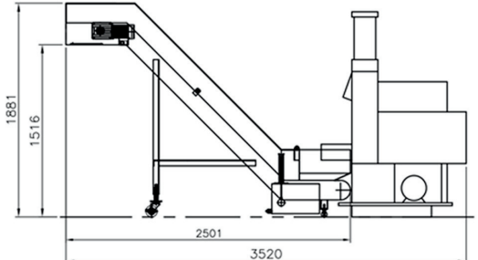
Finished Products Conveyor
