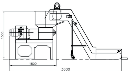
Dual Motors Shredder
